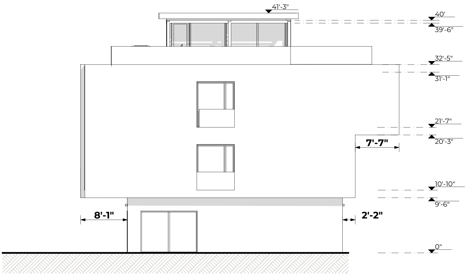
Right exterior elevation
