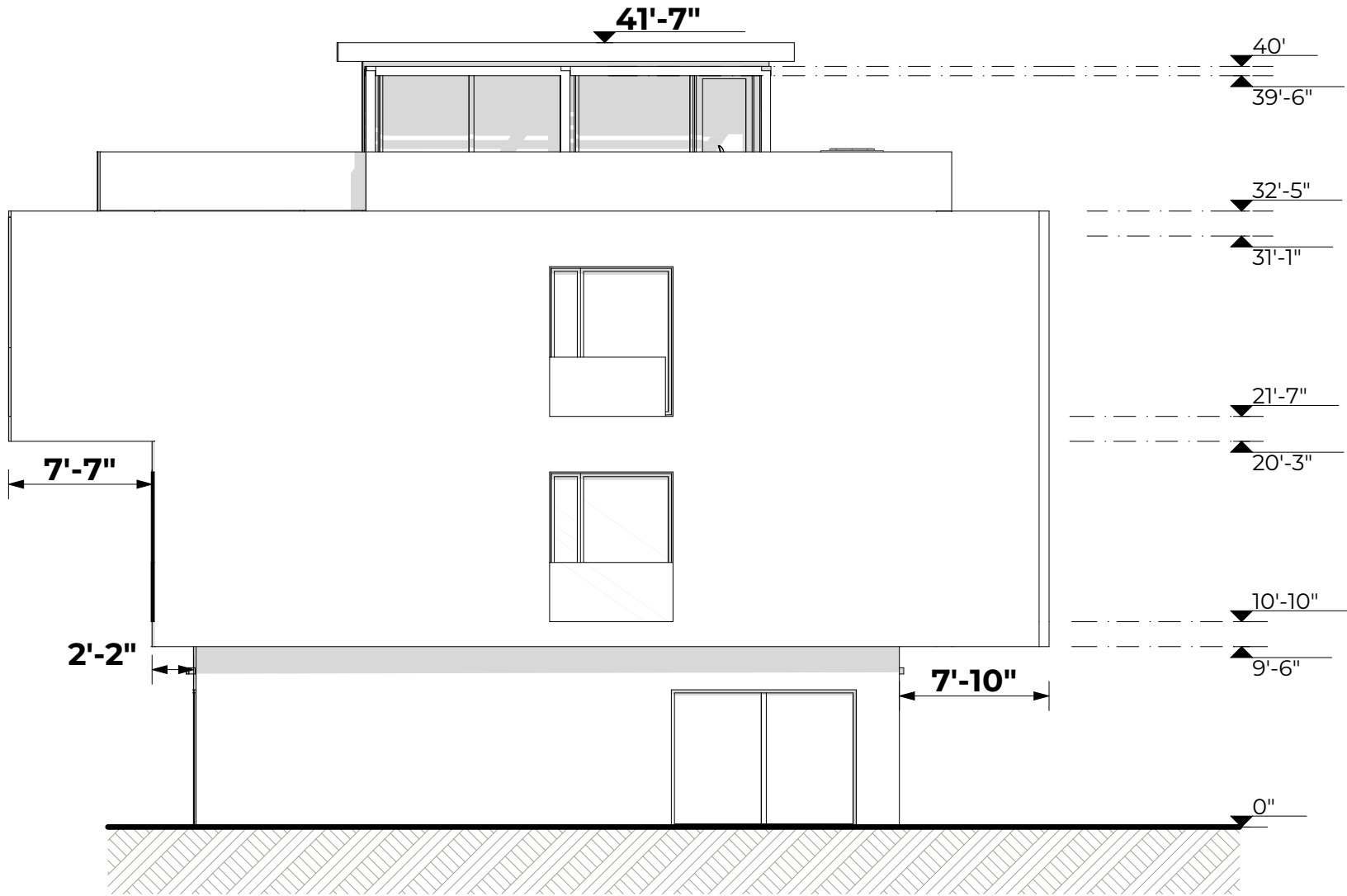
Left exterior elevation
